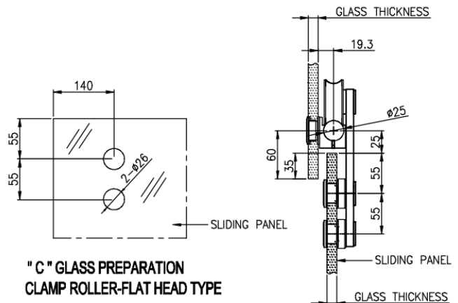
C) Clamp Roller (Glass to Glass)
