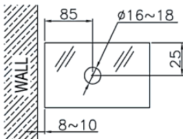
CARRIAGE ROLLER (STRAIGHT TYPE)
