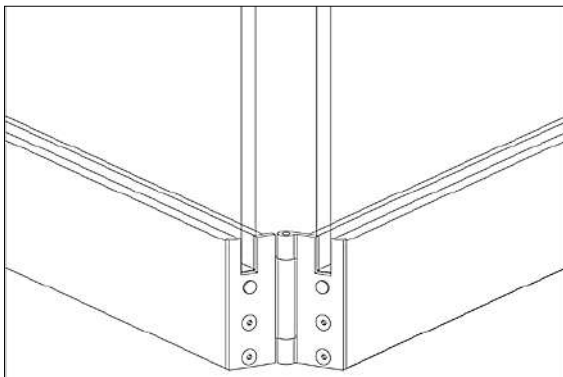
Bottom Rail c/w Hinge
