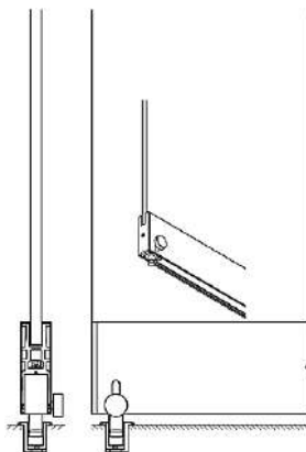
Bottom Rail c/w Latch
