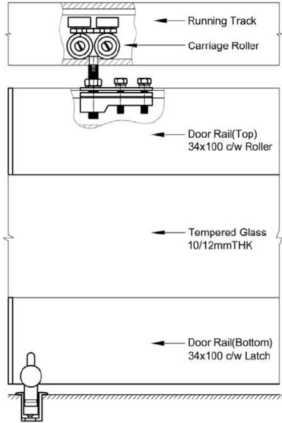
Top Rail c/w Carriage Roller
