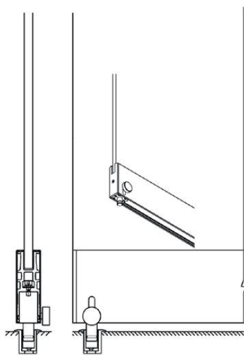
Sliding Panel c/w Thumb Push Latch
