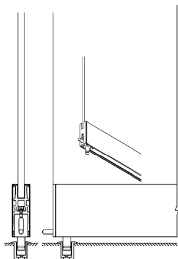
Sliding Panel c/w Security Latch
