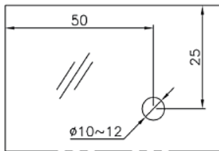
GLASS PREPARATION
