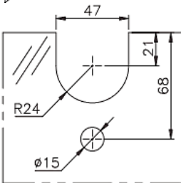
GLASS PREPARATION
