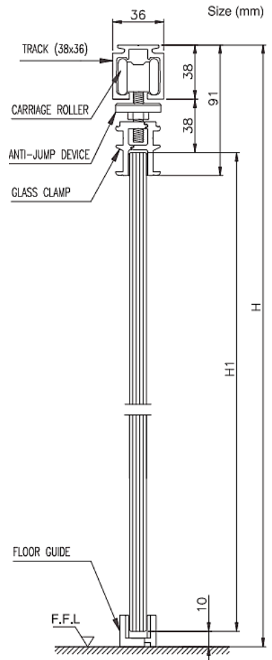
SECTIONAL DETAILS
