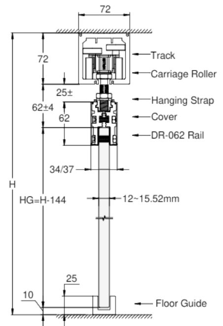
SECTIONAL DETAILS
