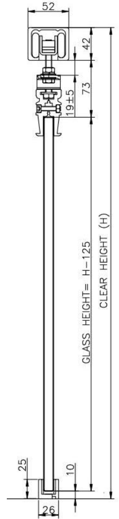
SECTIONAL DETAILS
