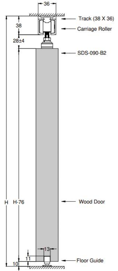
SECTIONAL DETAILS
