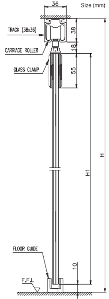
SECTIONAL DETAILS
