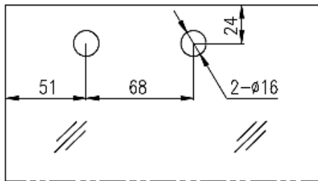
GLASS PREPARATION
