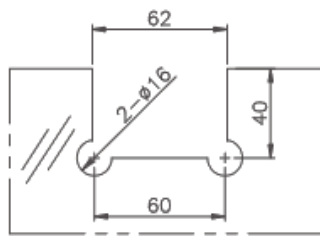
GLASS PREPARATION
