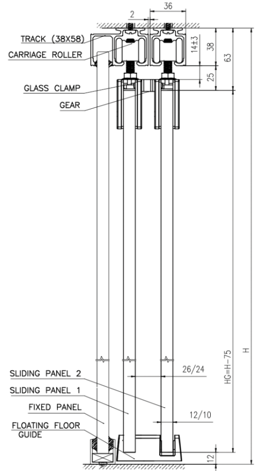
SECTIONAL DETAILS
