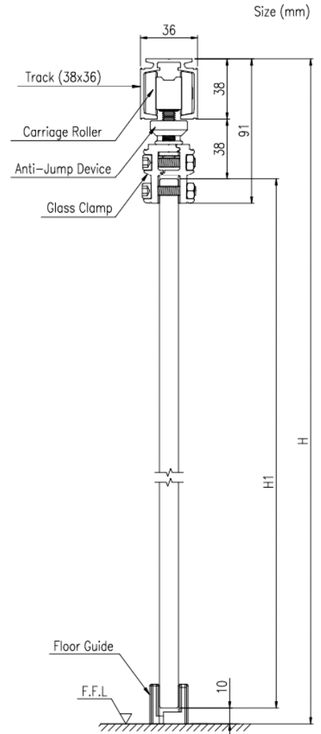
SECTIONAL DETAILS
