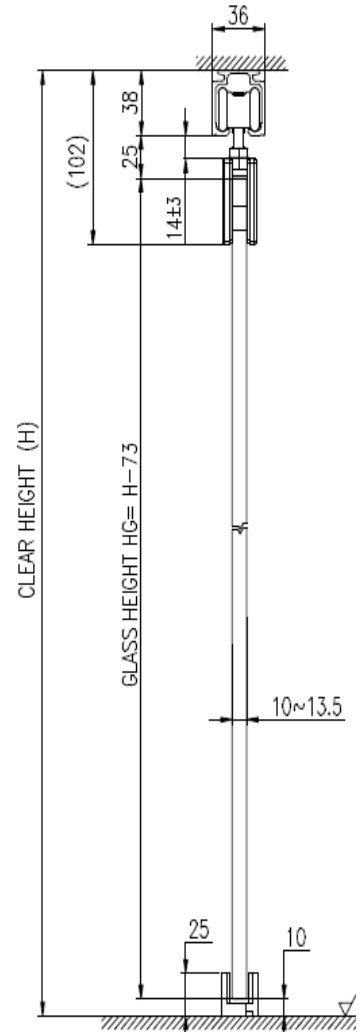
SECTIONAL DETAILS
