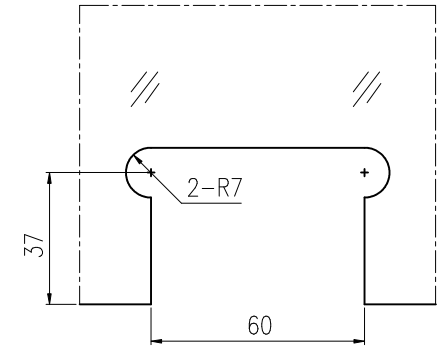
GLASS PREPARATION
