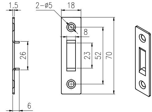
Wall Plate
